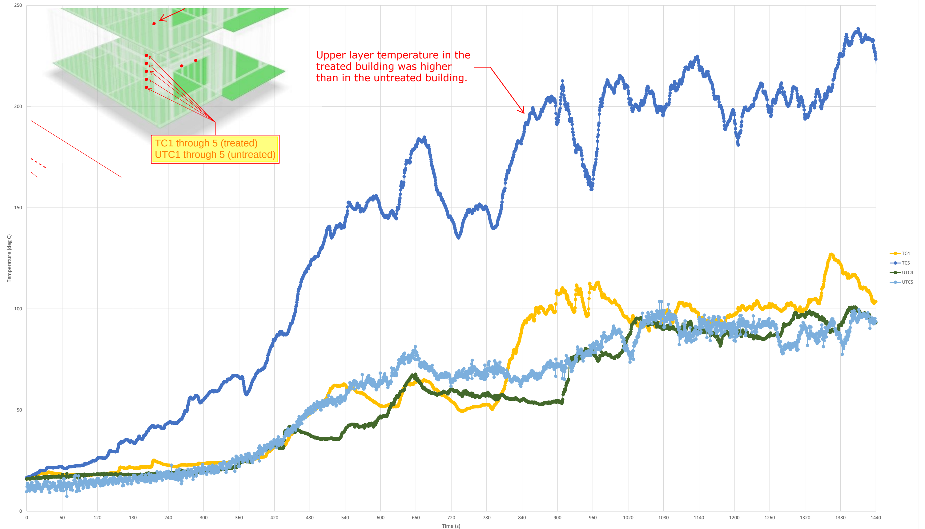
Comparison of upper layer temperatures prior to structure catching fire
